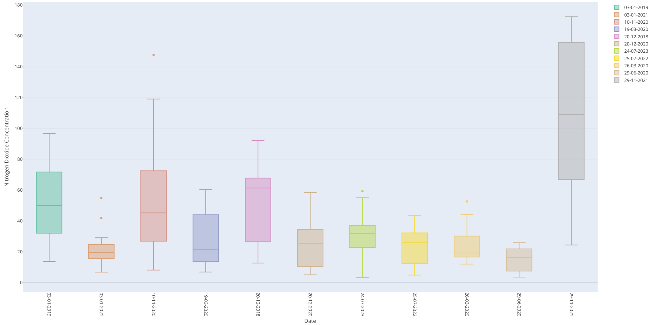
Distribution of Nitrogen Oxides as Nitrogen Dioxide by Date
